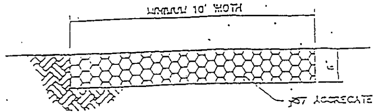
ELEVATION VIEW
