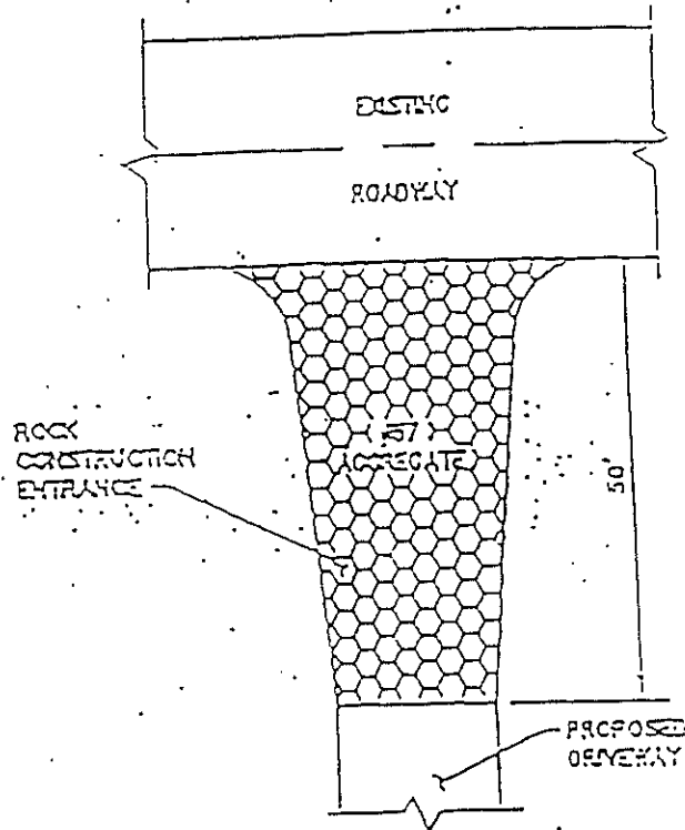
PLAN VIEW
